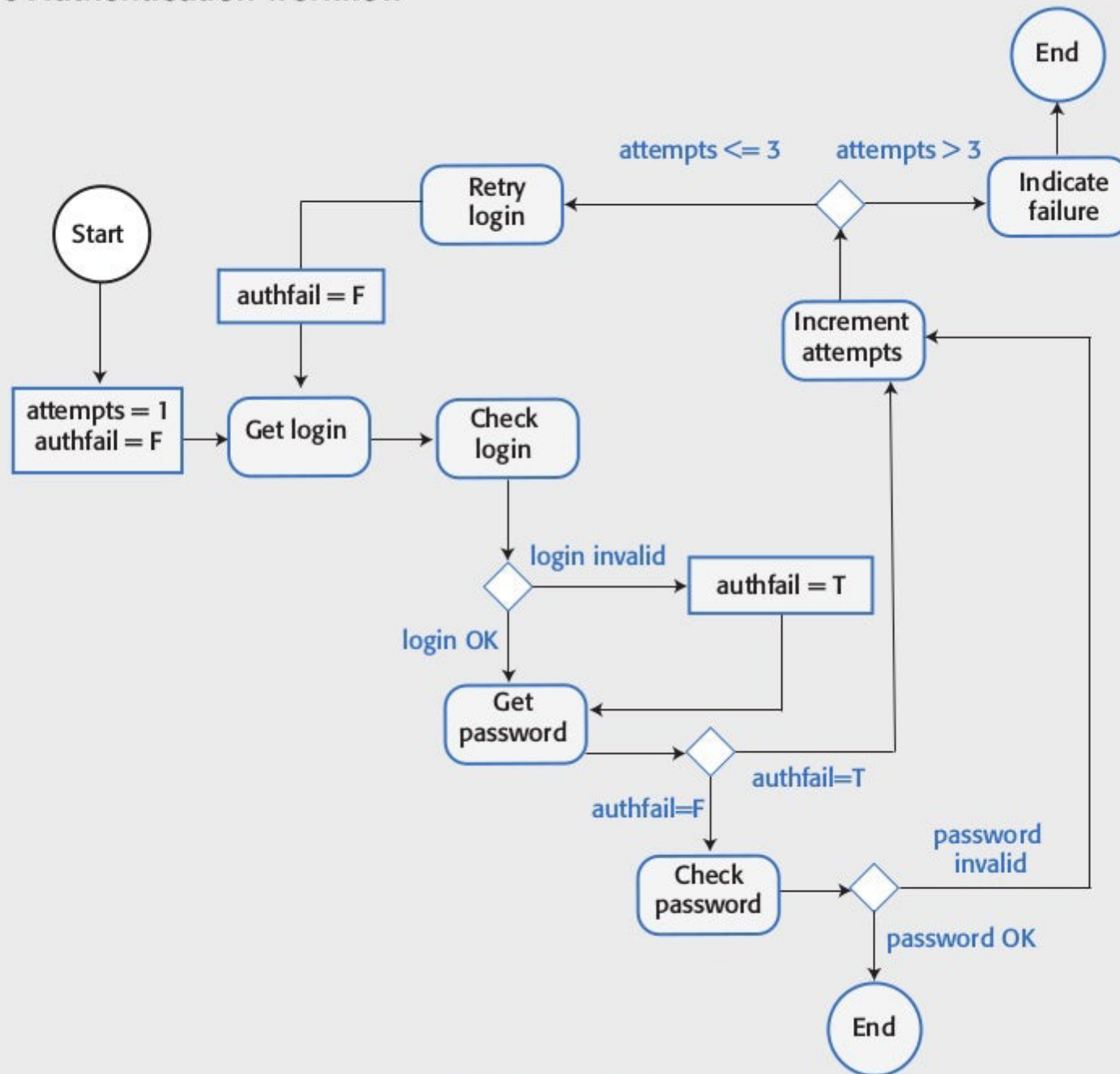
Figure 6.10 Authentication workflow
